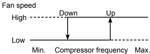
<Relation between compressor frequency and fan speed>
